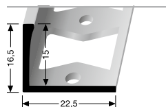
306 G PROFIL DOUBLE-K PERFORATED EDGE TRIM
