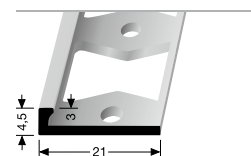
301 G PROFIL DOUBLE-K PERFORATED EDGE TRIM
