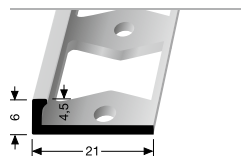
302 G PROFIL DOUBLE-K PERFORATED EDGE TRIM
