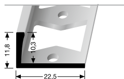
304 G PROFIL DOUBLE-K PERFORATED EDGE TRIM
