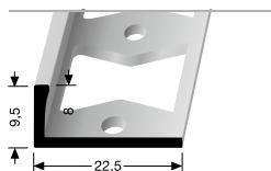
303 G PROFIL DOUBLE-K PERFORATED EDGE TRIM
