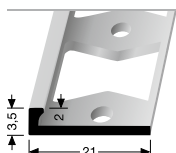
299 G PROFIL DOUBLE-K PERFORATED EDGE TRIM
