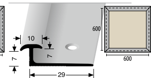
297 R RÁMEC REVIZE FLOOR ACCESS COVER FRAME
