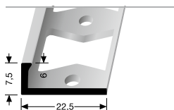
307 G PROFIL DOUBLE-K PERFORATED EDGE TRIM
